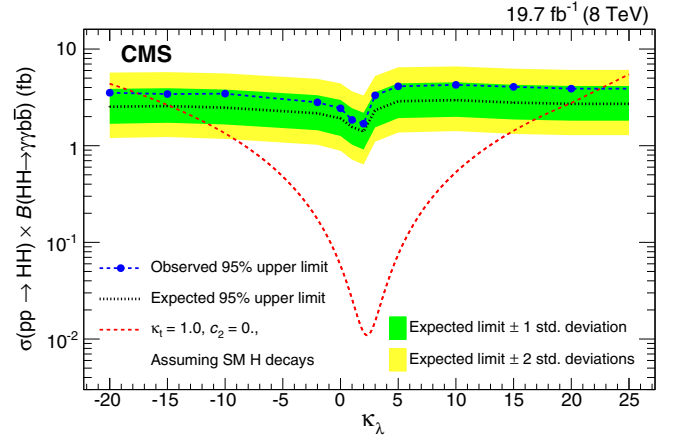
FIG. 10. Observed and expected 95% C.L. upper limits on the product of cross section and the branching fraction \sigma(pp \rightarrow HH)\mathcal{B}(HH \rightarrow \gamma\gamma b\bar{b}) for the nonresonant BSM analysis, performed by changing only \kappa_\lambda , while keeping all other parameters fixed at the SM predictions.
