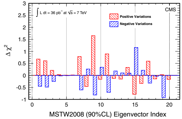
FIG. 4 (color online). The change in \chi^2 when comparing the Z rapidity differential cross section measurement with the predictions of the NLO MSTW2008 PDF set as each of the eigenvector input parameters is varied by \pm 90\% confidence level (CL) around its default value.
