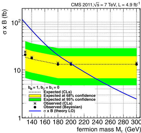
Fig. 5. The expected (dashed line) and observed (black points) exclusion limits at 95% confidence level on \sigma B as a function of the fermion mass M_\Sigma , assuming b_e = 1, b_\mu = 0, b_\tau = 0 (eS) for the signal. The solid (blue) curve represents the predictions of the LO type III seesaw models. The light (yellow) and dark (green) shaded areas represent, respectively, the 1 standard deviation (68% CL) and 2 standard deviations (95% CL) limits on the expected results obtained from MC pseudo-experiments, which reflect the combined statistical and systematic uncertainties of the SM contributions. The asterisks and the black points show, respectively, the observed limits computed following a frequentist method based on the CLs criterion and a Bayesian approach.
