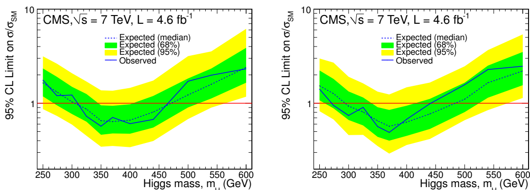
Figure 4. The ratio R of the 95% CL cross section upper limit \sigma to the SM Higgs boson production cross section \sigma_{SM} as a function of the Higgs boson mass m_H for the cut-based (left) and shape-based (right) analyses.
