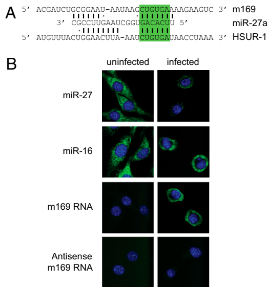
Fig. 6. Sequence alignment of miR-27-binding sites in HSUR-1 and m169 and cytoplasmic localization of miR-27 and m169 in NIH 3T3 cells. (A) Complementarity of m169 and HSUR-1 to miR-27; green box indicates the seed site. (B) In situ detection of DIG-labeled probes against miR-27, miR-16, m169, and antisense m169 in NIH 3T3 cells, uninfected or at 16 h post-infection. DIG-labeled probes were detected by FITC-tyramide amplification (green) and overlaid on nuclear DAPI signal (blue). Images are representative of three independent experiments.
