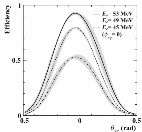
Fig. 4 Efficiencies of the trigger directional match selection versus relative angles. The bands around the curves show the uncertainties ( 1\sigma )
