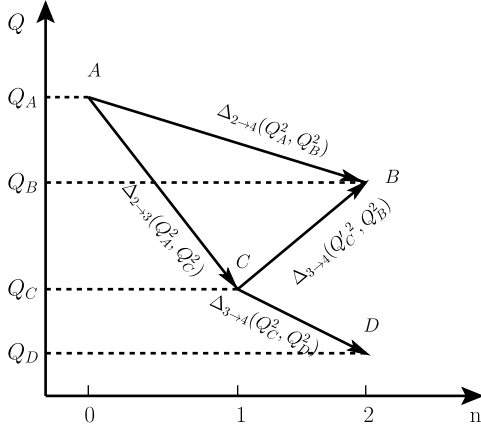
Fig. 1. Illustration of scales and Sudakov factors in strongly ordered (ACD), smoothly (un)ordered (ACB), and direct 2 \rightarrow 4 (AB) branching processes, as a function of the number of emitted partons, n .
