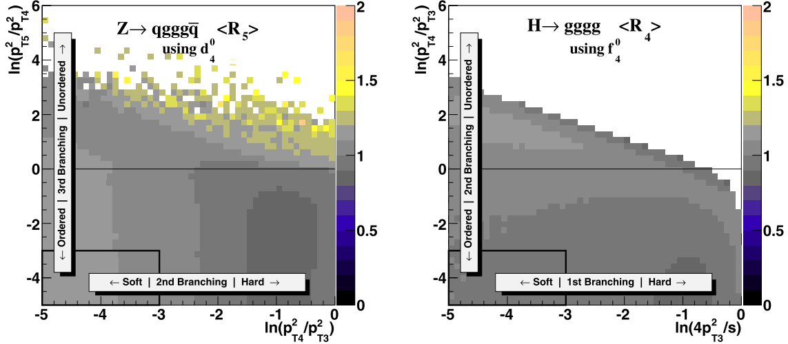
Fig. 2. Mean value of R_5 (left) and R_4 (right) differentially over phase space, with n -parton clustering scales p_{Tn} \equiv p_T(\Phi_n) . Note that the “top edges” of the phase spaces correspond to hard configurations that are not logarithmically enhanced.
