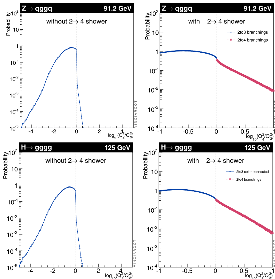
Fig. 3. Top left: the ratio of sequential clustering scales Q_4/Q_3 for a strongly ordered 2 \rightarrow 3 shower, for Z \rightarrow qgg\bar{q} (on log-log axes). Top right: closeup of the region around Q_4/Q_3 \sim 1 , with 2 \rightarrow 4 branchings included. Bottom row: the same for H \rightarrow gggg .
