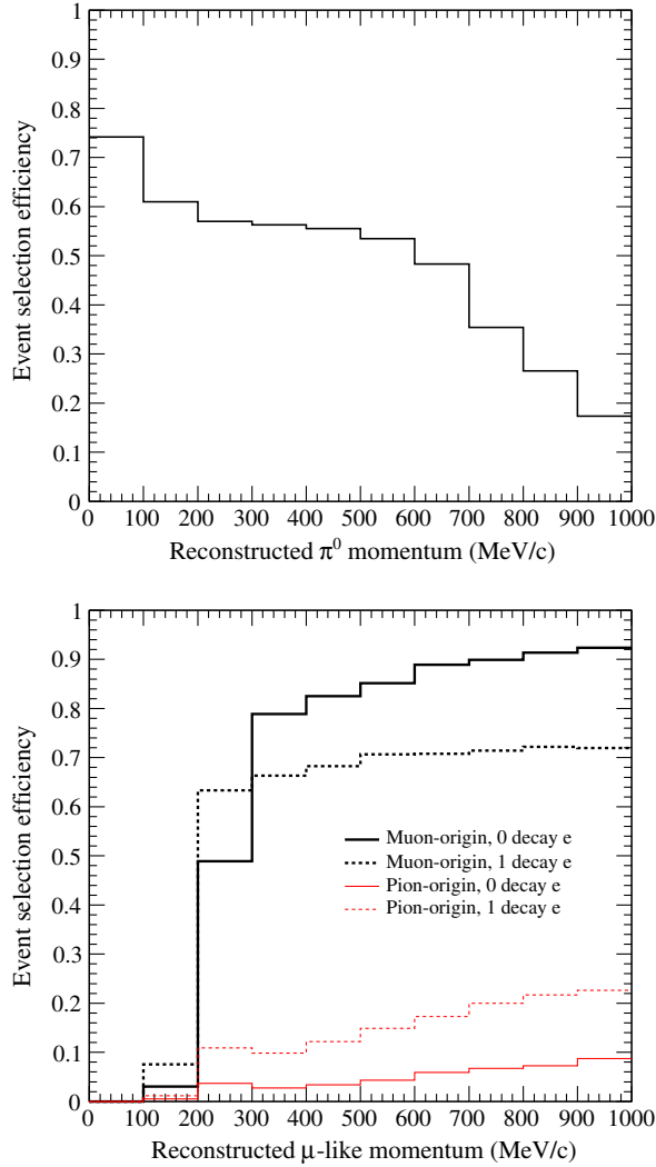
FIG. 1 (color online). Event selection efficiencies for atmospheric neutrino MC as a function of reconstructed momentum for n \rightarrow \bar{\nu}\pi^0 selection cuts (top) and p \rightarrow \bar{\nu}\pi^+ selection cuts (bottom). For the \pi^+ sample, all momenta are calculated assuming a muon hypothesis. The atmospheric neutrino events that make up the background for the p \rightarrow \bar{\nu}\pi^+ mode are treated separately in the spectrum fit according to their origin.
