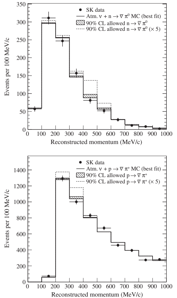
FIG. 3. Reconstructed momentum for 172.8 kt · yr of SK-I + II + III data (black dots), best fit result of atmospheric neutrino plus nucleon decay MC simulation (solid line), and the 90% C.L. allowed amount of nucleon decay (hatched histogram) for n \rightarrow \bar{\nu}\pi^0 (top) and p \rightarrow \bar{\nu}\pi^+ (bottom). The dashed line shows how a positive signal of nucleon decay would look, corresponding to five times the limit we set on the decay partial lifetimes. The p \rightarrow \bar{\nu}\pi^+ nucleon decay contribution in the bottom figure is reconstructed at lower momentum than the expected value (458.8 MeV/ c ) because a muon hypothesis is assumed in the reconstruction.
