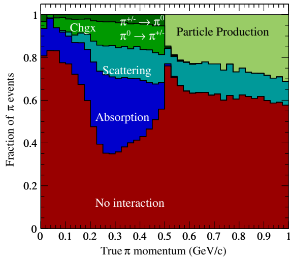
FIG. 2 (color online). Cumulative fractions of nuclear effects for \pi^0 as a function of true \pi^0 momentum for atmospheric neutrino interactions. The fractions of events that undergo charge exchange, multiple particle production, scattering, and absorption are shown by various shades as labeled. Pions that exit the nucleus without experiencing any nuclear effect are indicated by the portion labeled “No interaction.”
