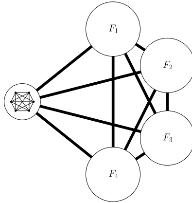
Fig. 1. The gadget graph G_0 in Lemma 2.5 for k = 6 . A thick line indicates that the vertices of the corresponding sets are pairwise connected.
