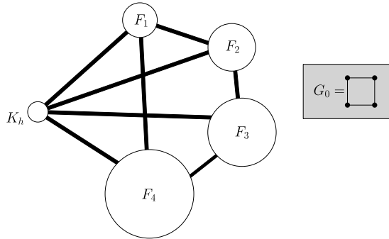
Fig. 4. An illustration of G(h, G_0, F_1, F_2, F_3, F_4) when G_0 = C_4 . A thick line indicates that the vertices of the corresponding sets are pairwise connected.
