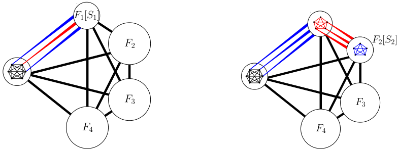
(a) Colour-focusing between H = K_6 and F_1 .
