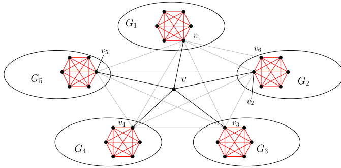
Fig. 3. An example of the graph G in Lemma 2.7 for k = 6 .
