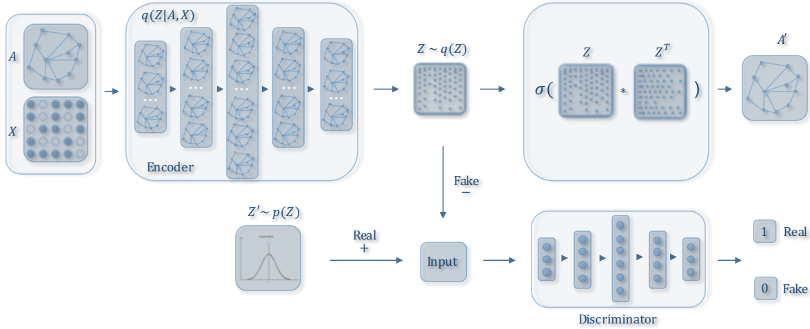
Figure 1: The architecture of the adversarially regularized graph autoencoder (ARGA). The upper tier is a graph convolutional autoencoder that reconstructs a graph A from an embedding Z which is generated by the encoder which exploits graph structure A and the node content matrix X . The lower tier is an adversarial network trained to discriminate if a sample is generated from the embedding or from a prior distribution. The adversarially regularized variational graph autoencoder (ARVGA) is similar to ARGAs except that it employs a variational graph autoencoder in the upper tier (See Algorithm 1 for details).
