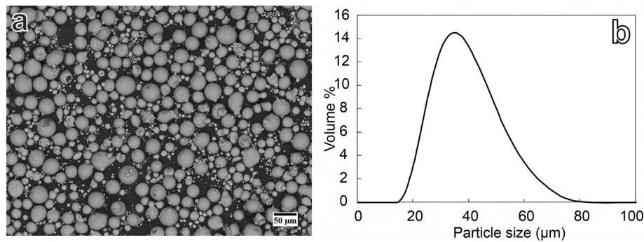
Fig. 1. (a) SEM image showing powder morphology and (b) particle size distribution.
