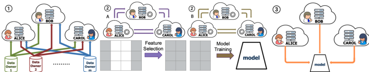
Figure 1. Overview of private feature selection and model training in 3PC setting with computing servers (parties) Alice , Bob , and Carol .
