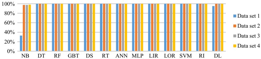
Fig. 2 Non-fraud detection rates of data set 1–4
