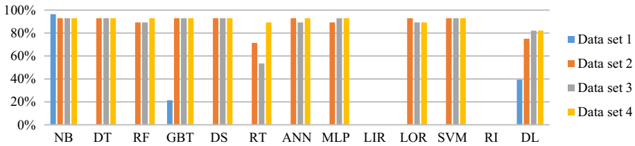
Fig. 1 Fraud detection rates of data sets 1–4
